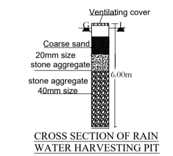
CROSS SECTION OF RAIN WATER HARVESTING PIT
